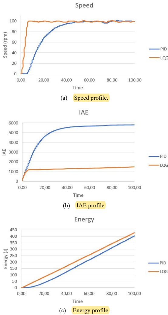
Figure 7. System responses in load test.
