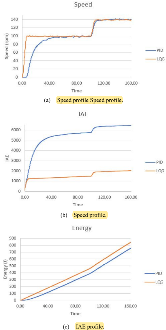
Figure 8. System responses in tracking test.
