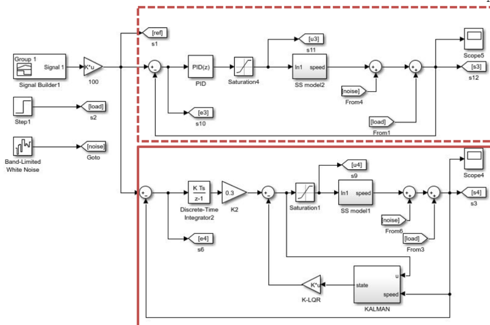
Figure 5. Block diagram of PID and LQR control in Simulink.
